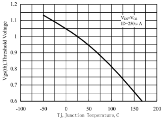
Figure 11 Typical Theshold Voltage vs Junction Temperature
