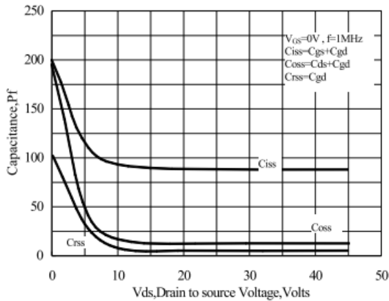
Figure 13 Typical Capacitance vs Drain to Source Voltage
