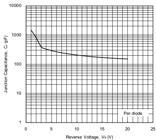
Fig. 4 - Junction Capacitance
