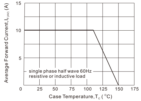
Fig.2 - Forward Current Derating Curve (total device)
