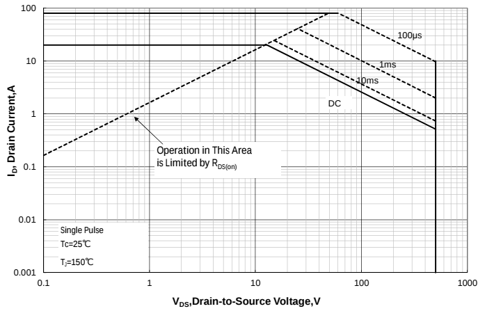
Figure 1 Maximum Forward Bias Safe Operating Area
