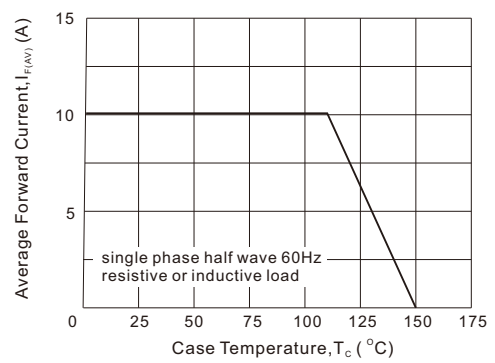
Fig. 1 - Forward Current Derating Curve (total device)
