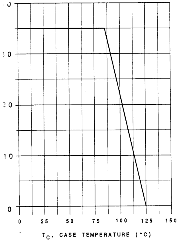
MAXIMUM ON-STATE CURRENT vs. CASE TEMPERATURE
