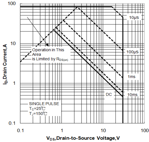
Figure 1. Maximum Safe Operating Area
