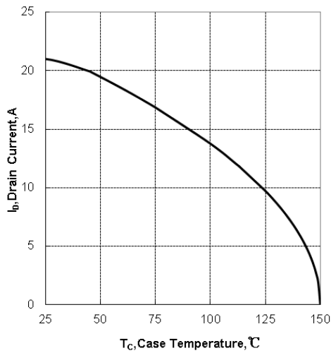
Figure 3. Maximum Continuous Drain Current vs Case Temperature
