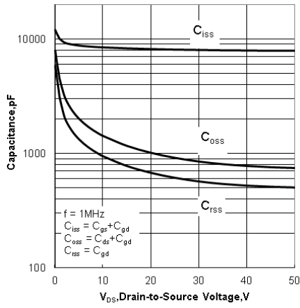
Figure12. Capacitance Characteristics
