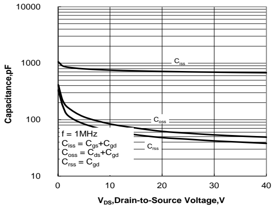
Figure 12. Capacitance Characteristics
