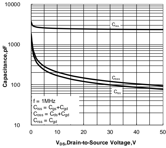
Figure 12. Capacitance Characteristics
