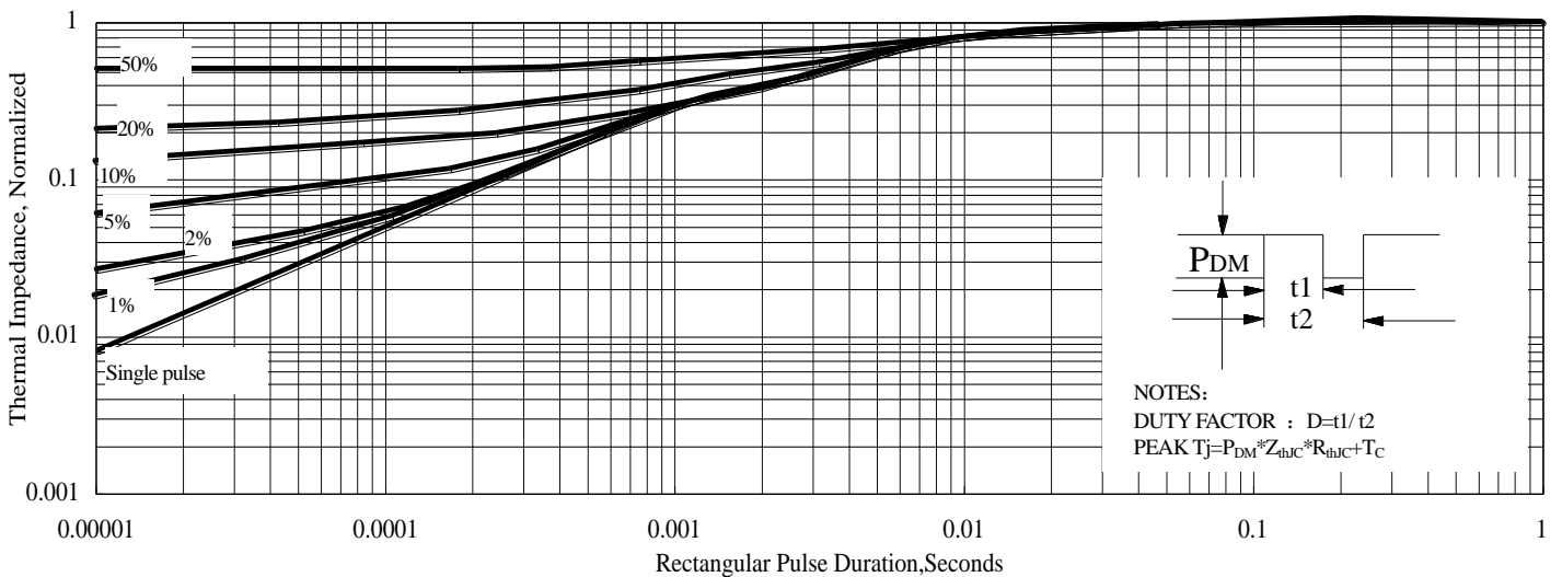
Figure 5 Maximum Effective Thermal Impedance, Junction to Ambient
