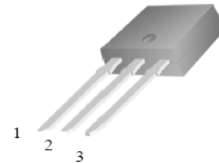
1.Gate 2.Drain 3.Source
