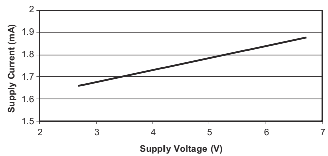
Figure 6. Supply Current vs. Supply Voltage
