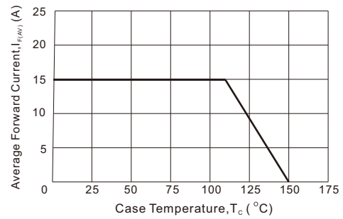
Fig. 4 - Forward Current Derating Curve (per diode)
