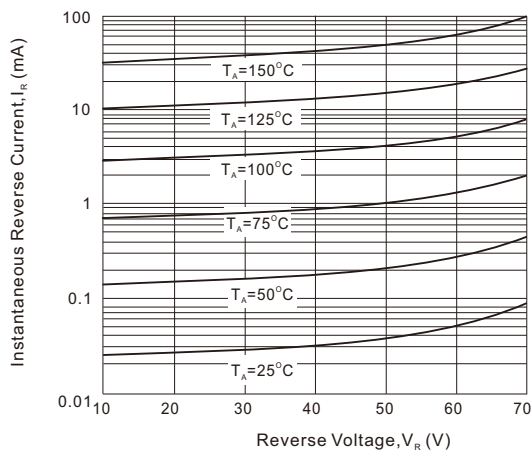
Fig. 3 - Reverse Characteristics (per diode)
