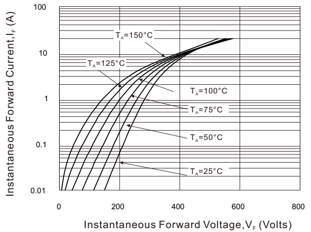
Fig. 2 - Instantaneous Forward Characteristics (per diode)
