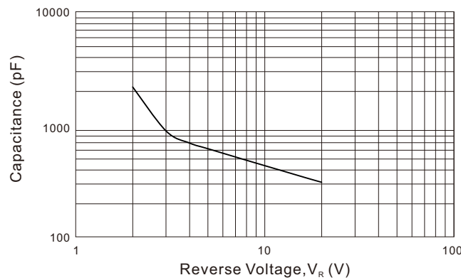
Fig. 5 -Junction Capacitance
