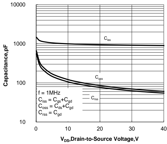
Figure 12. Capacitance Characteristics
