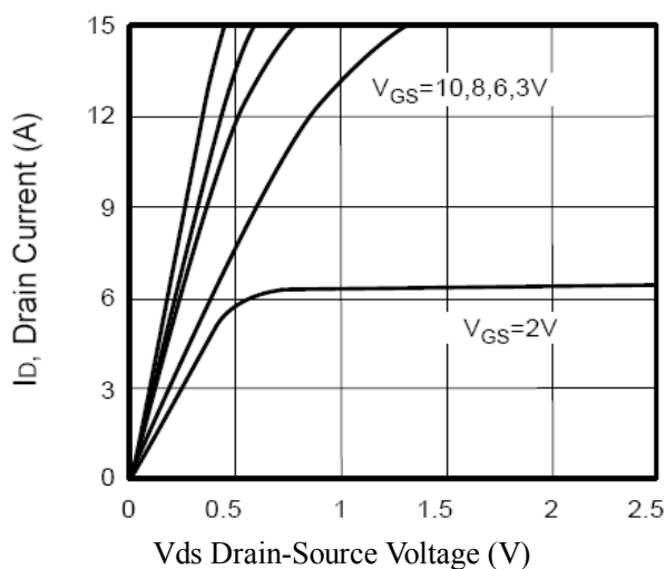
Figure3. Output Characteristics
