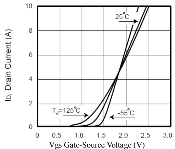
Figure4. Transfer Characteristics
