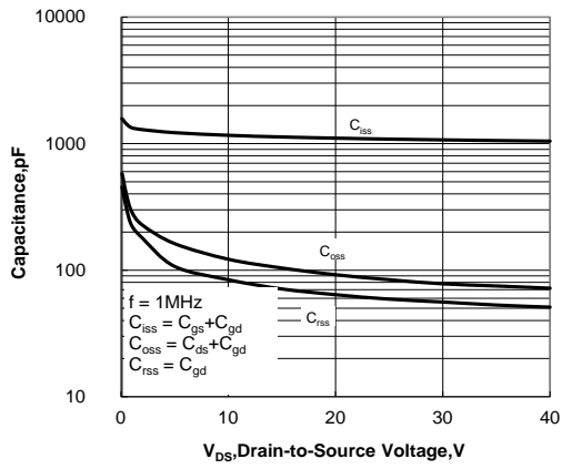
Figure 12. Capacitance Characteristics
