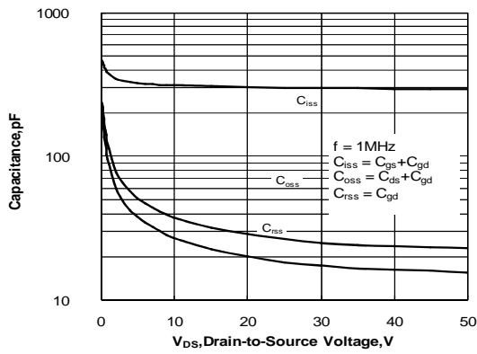
Figure 12. Capacitance Characteristics
