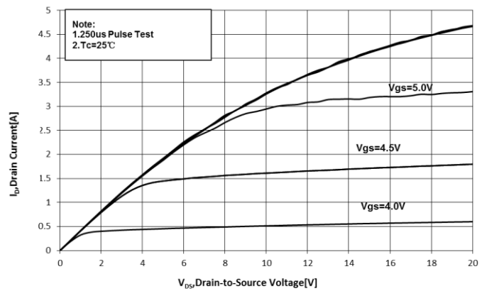
Figure 4 Typical Output Characteristics
