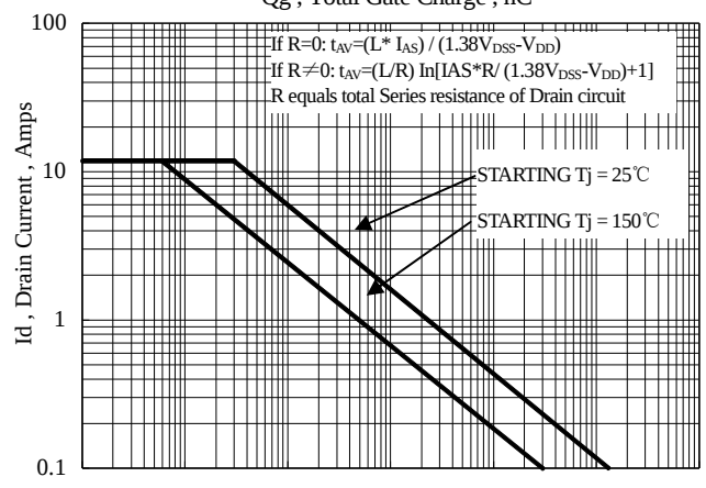
Figure 16 Unclamped Inductive Switching Capability tAV, Time in Avalanche, Seconds
