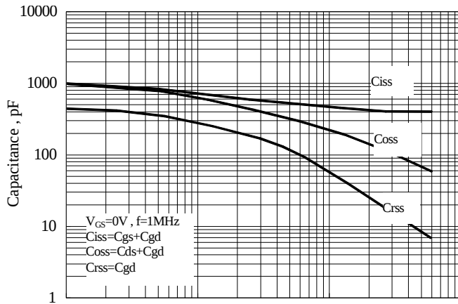
Figure 13 Typical Capacitance vs Drain to Source Voltage Vds, Drain to Source Voltage, Volts
