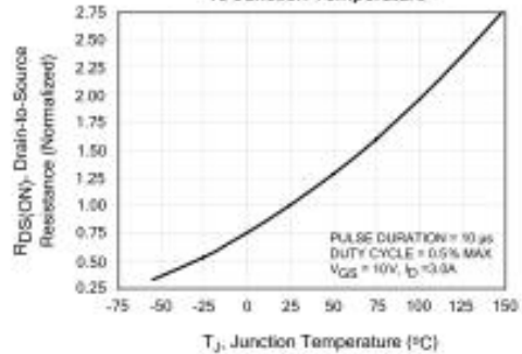
Figure 10. Typical Drain-to-Source ON Resistance vs Junction Temperature
