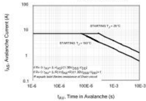
Figure 8. Unclamped Inductive Switching Capability
