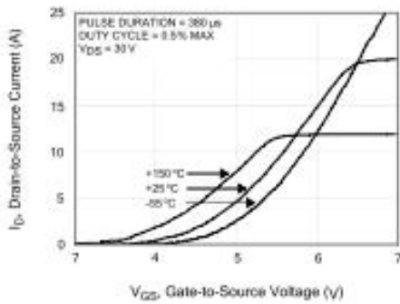
Figure 7. Typical Transfer Characteristics
