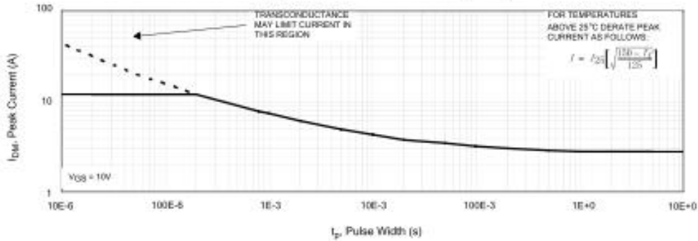
Figure 6. Maximum Peak Current Capability
