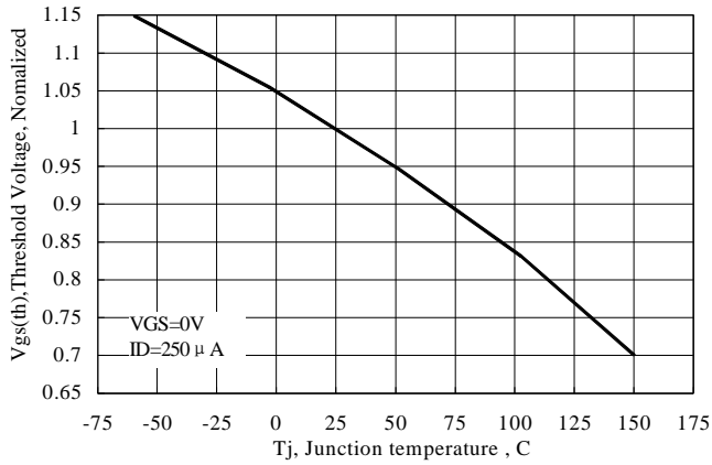
Figure 11 Typical Theshold Voltage vs Junction Temperature
