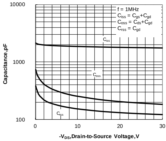
Figure 12. Capacitance Characteristics
