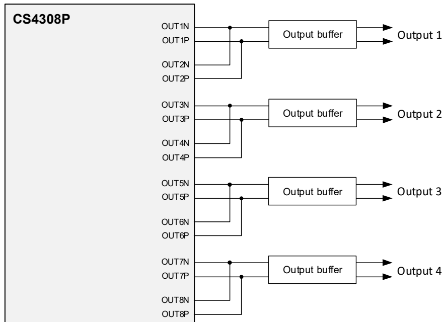
Figure 4-2. Output Summing
