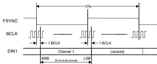
Figure 4-31. I 2 S Data Format
