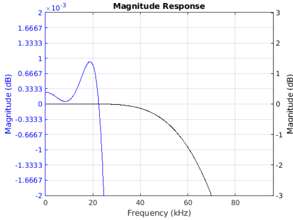
Figure 7-43. Passband Magnitude
