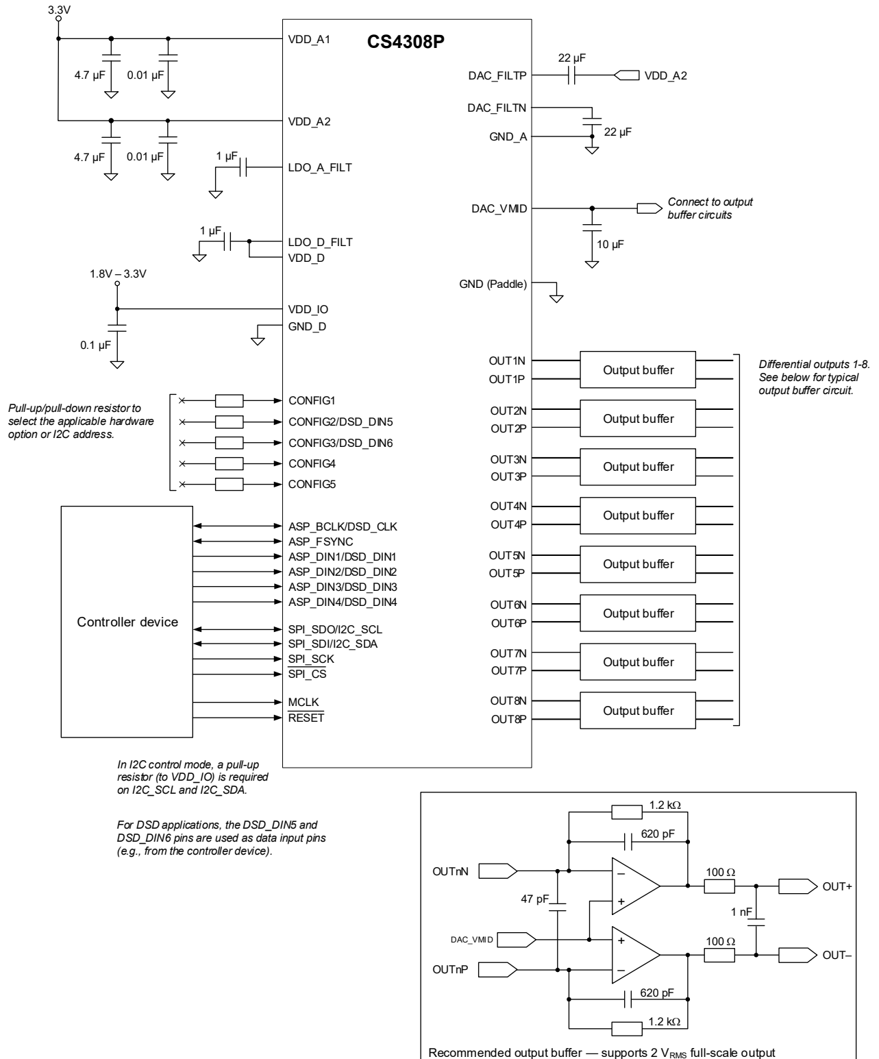
Figure 2-1. Typical Connections
