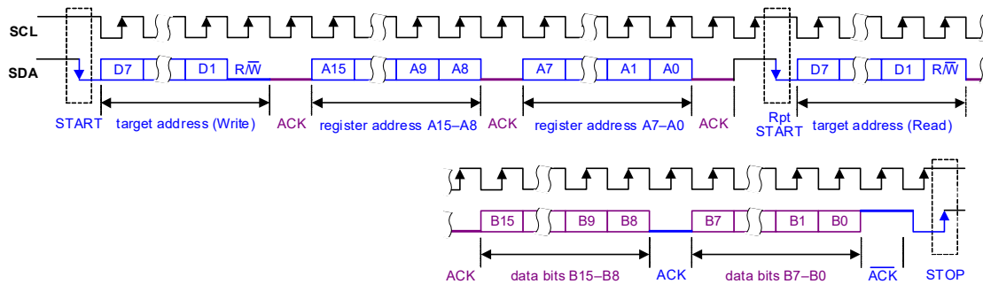
Figure 4-41. Control Interface I 2 C Register Read
