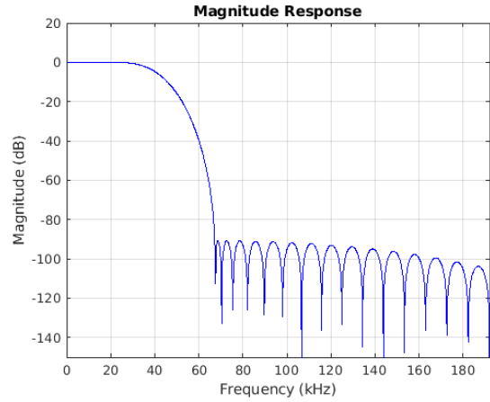
Figure 7-26. Stopband Magnitude
