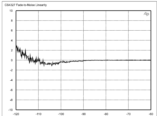
Figure 18. Fade-to-Noise Linearity
