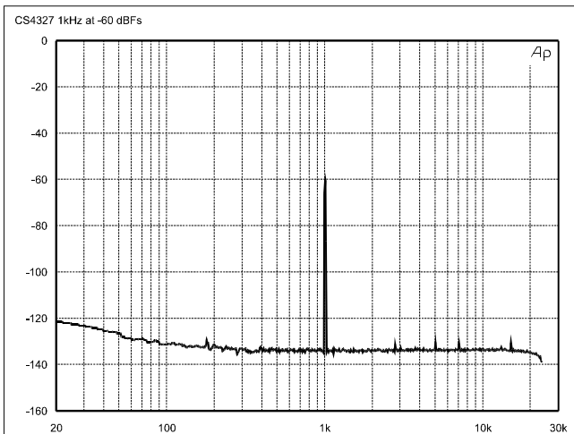
Figure 17. -60 dBFS FFT
