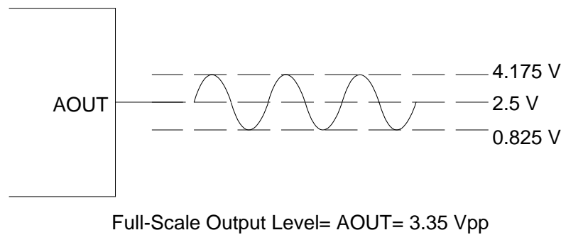
Figure 19. Full-Scale Output
