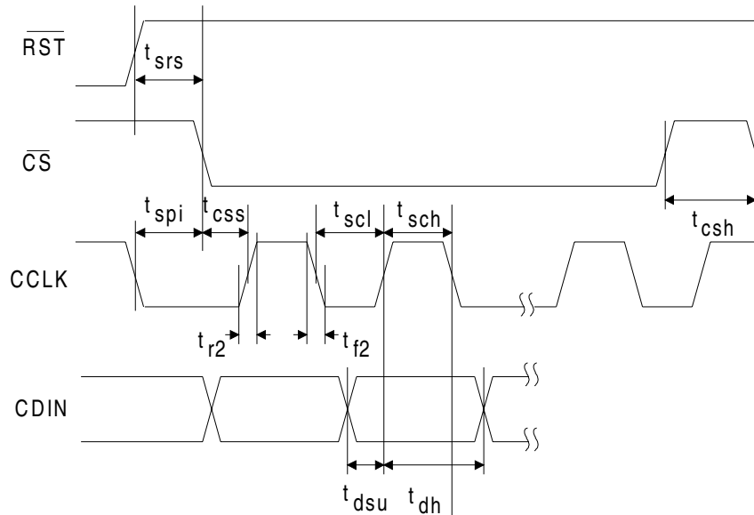
Figure 4. Control Port Timing - SPI Format
