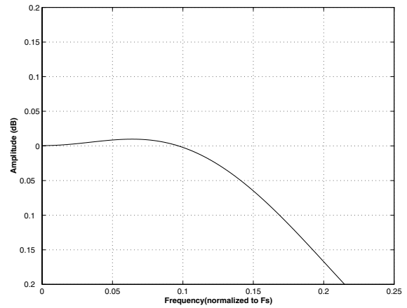
Figure 28. Quad Speed (fast) Passband Ripple
