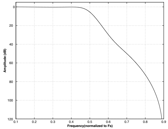
Figure 30. Quad Speed (slow) Transition Band
