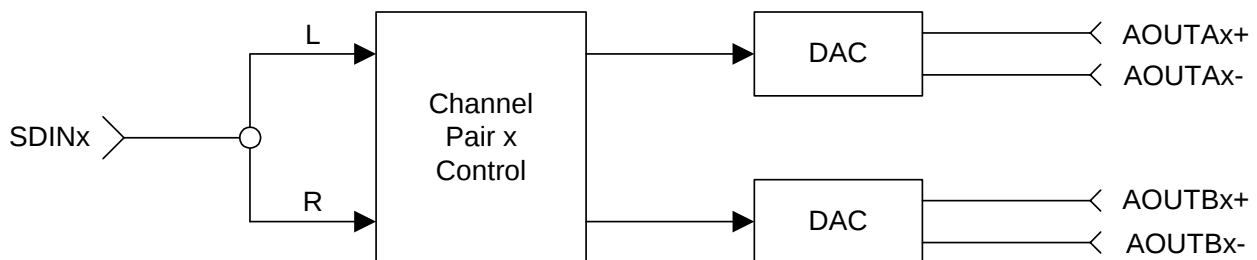
Figure 40. Channel Pair Routing Diagram (x = Channel Pair 1, 2, 3, or 4)
