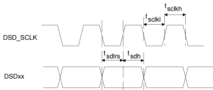
Figure 3. Direct Stream Digital - Serial Audio Input Timing
