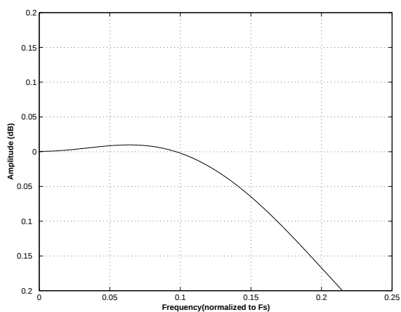
Figure 46. Quad-Speed (fast) Passband Ripple
