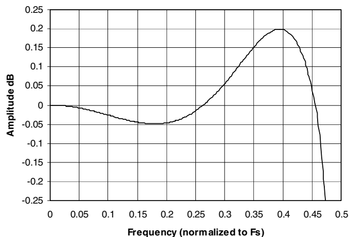
Figure 22. Double-Speed Frequency Response
