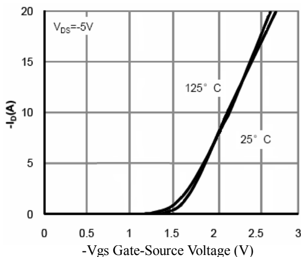
Figure4. Transfer Characteristics
