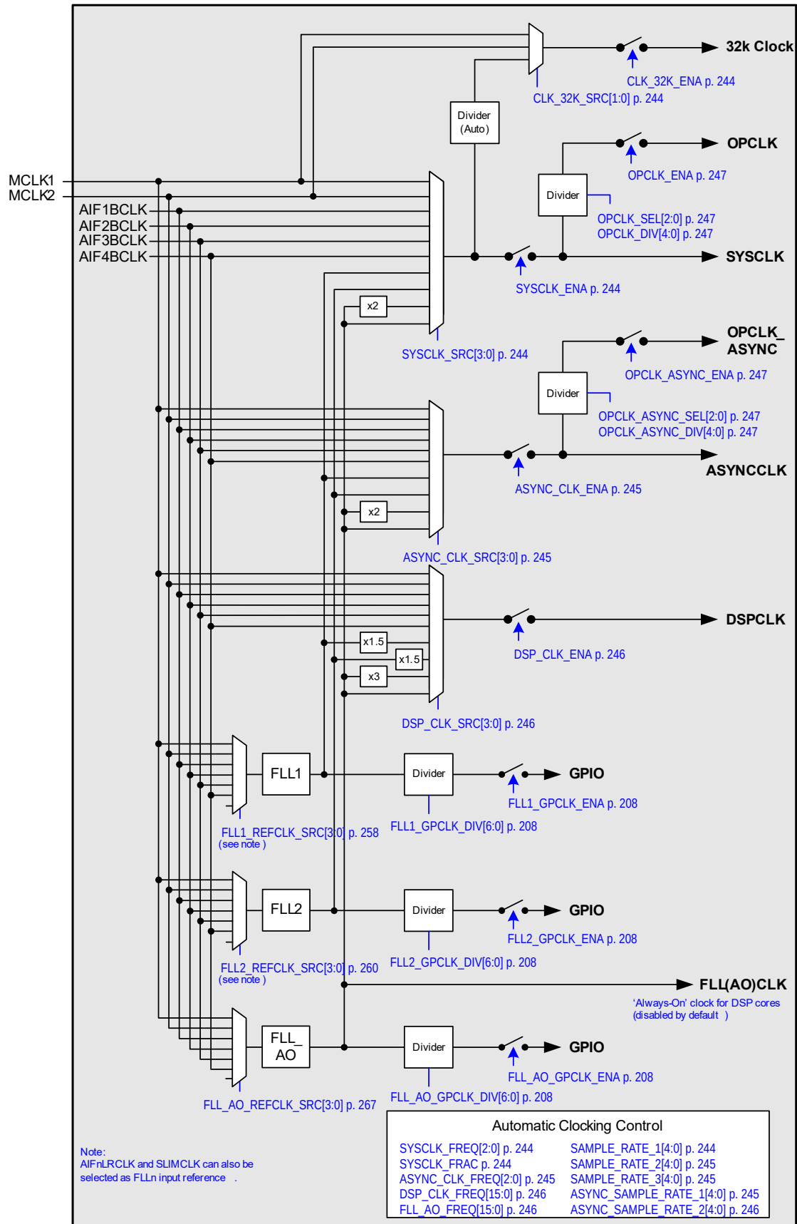
Figure 4-63. System Clocking
