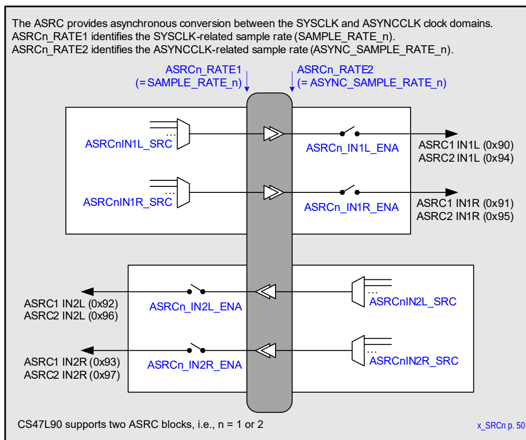
Figure 4-28. Asynchronous Sample-Rate Converters (ASRCs)
