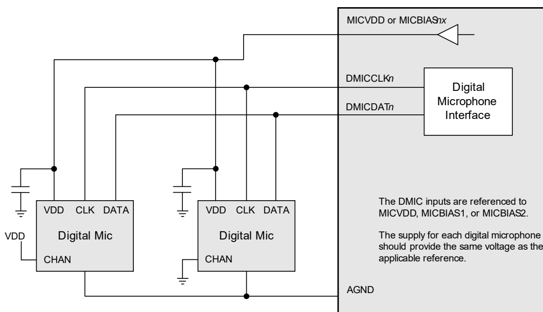
Figure 4-9. DMIC Input
