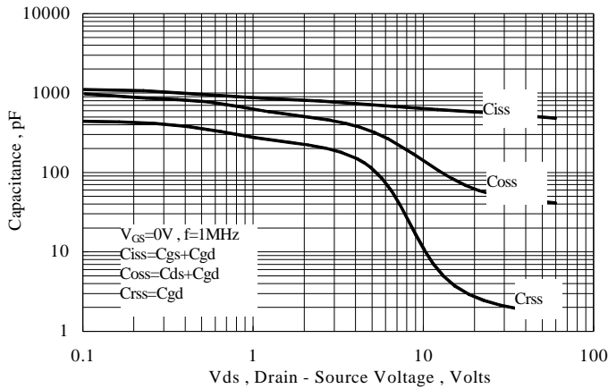
Figure 13 Typical Capacitance vs Drain to Source Voltage
