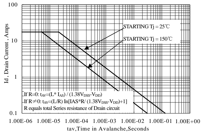
Figure 16 Unclamped Inductive Switching Capability
