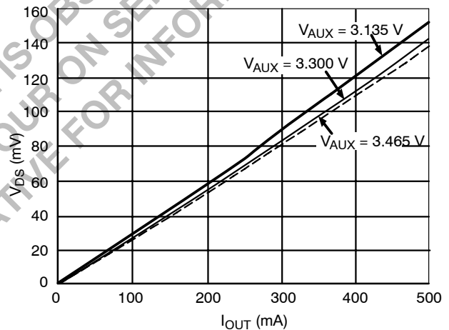
Figure 26. PFET V_{DS} vs. I_{OUT}
