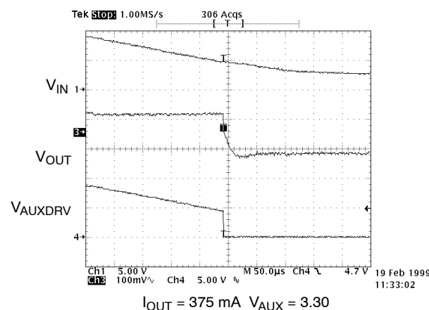
Figure 15. Power-Down, V_{AUX} = 3.3 \text{ V} . Again, Note \Delta V = I R_{DS(ON)} \approx 130 \text{ mV}
