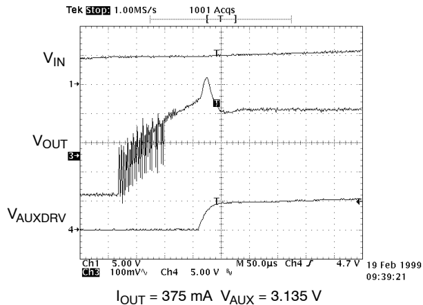
Figure 16. Power-Up, V_{AUX} = 3.135 V. The “Oscillatory Performance” Mode Lasts Longer Because the Difference Between V_{AUX} and 3.3 is Greater
