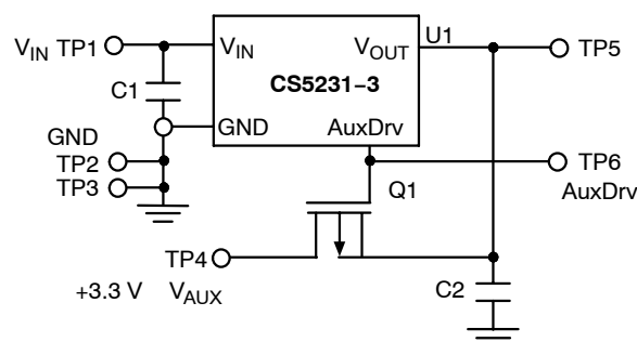
Figure 22. Application Circuit Schematic
