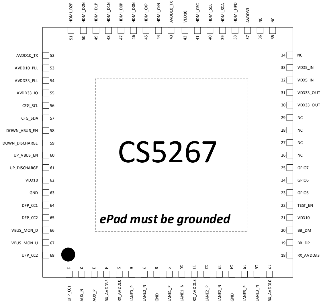
Figure 3-1 CS5267AN Pin Layout
