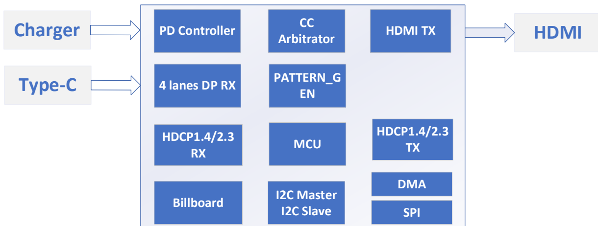
Figure 1-1 CS5267AN Block Diagram
