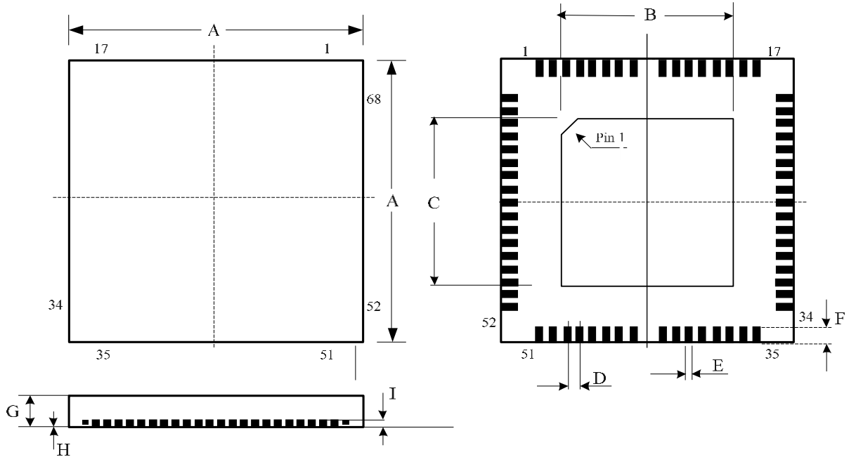
Figure 5-1 CS5267AN Package Outline (QFN68 Leads 8x8mm 2 )
