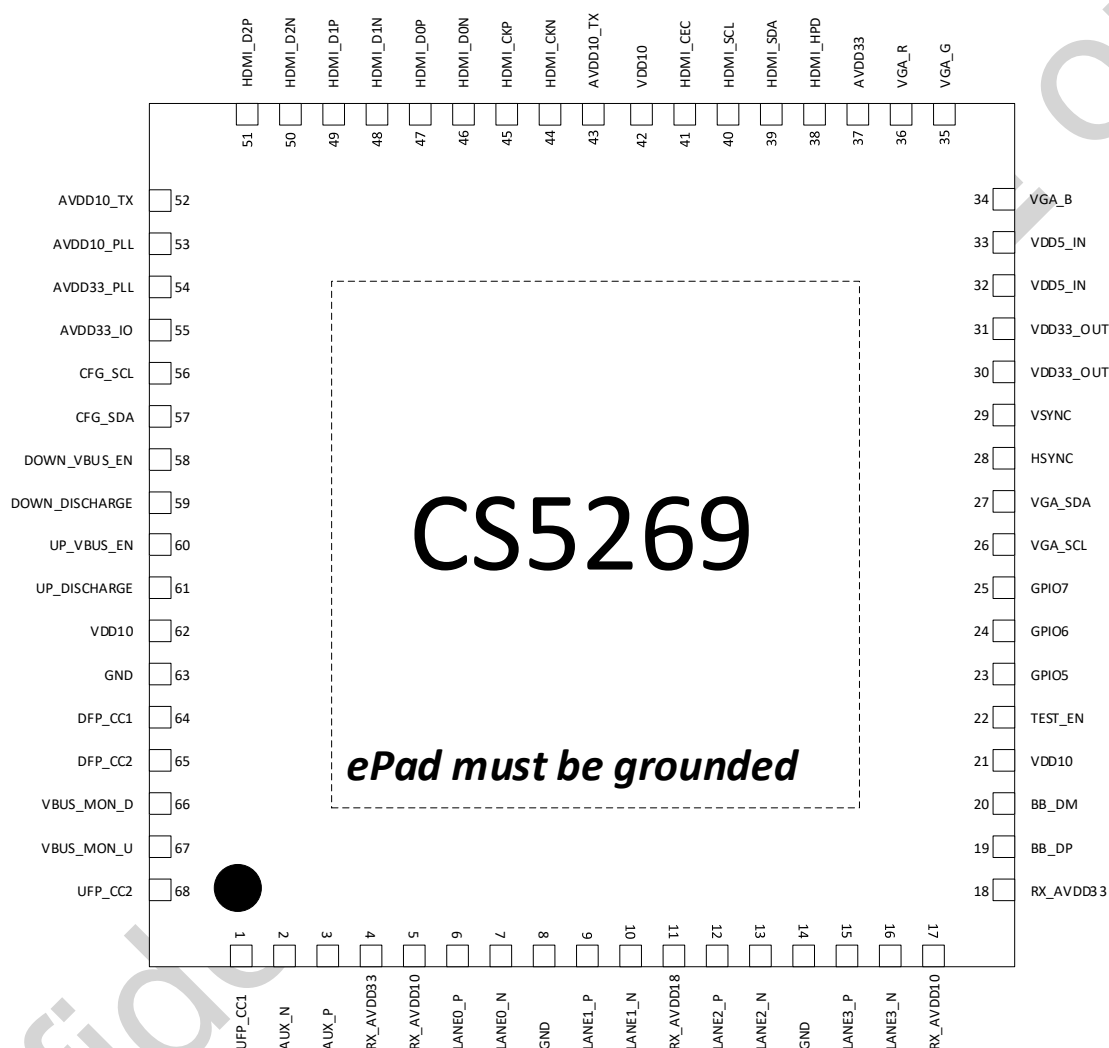
Figure 3-1 CS5269AN Pin Layout
