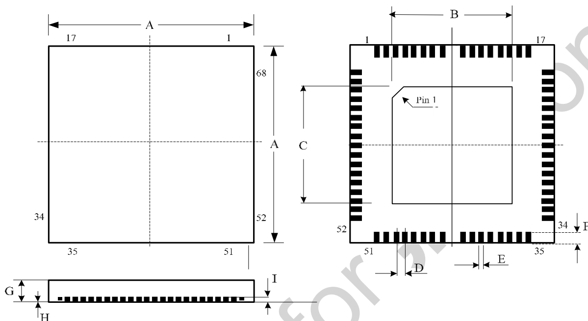
Figure 5-1 CS5269AN Package Outline (QFN68 Leads 8x8mm2)
