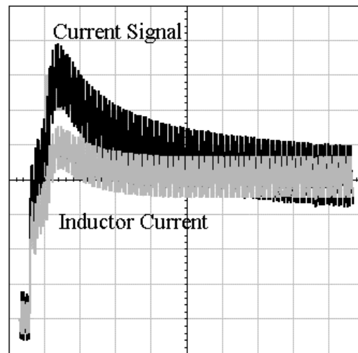
Figure 12. Inductive Sensing Waveform During a Load Step with Fast RC Time Constant (50 \mu\text{s}/\text{div} )
