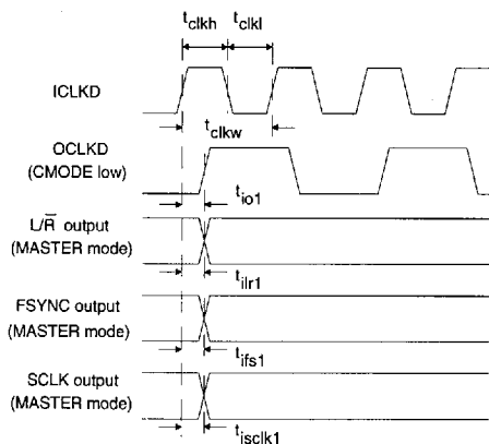
ICLKD to Outputs Propagation Delays (CMODE low)
