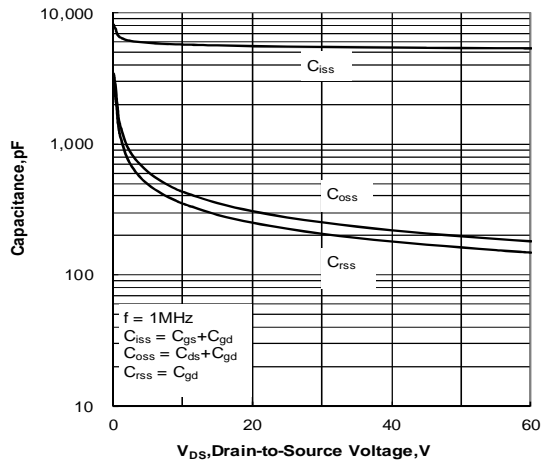
Figure 12. Capacitance Characteristics
