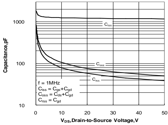
Figure 12. Capacitance Characteristics
