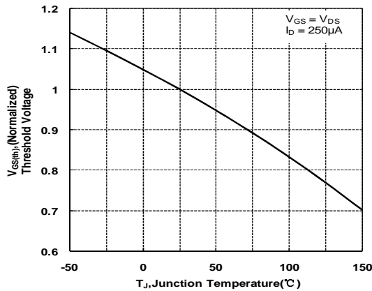
Figure 10. Normalized Threshold Voltage vs Junction Temperature
