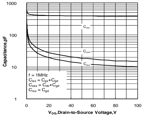
Figure 12. Capacitance Characteristics
