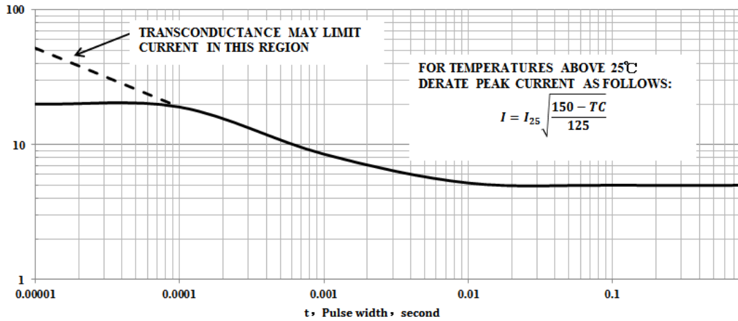
Figure 6 Maximum Peak Current Capability
