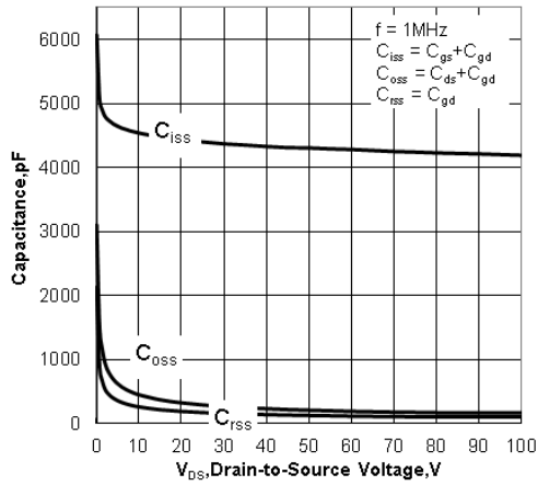
Figure12. Capacitance Characteristics
