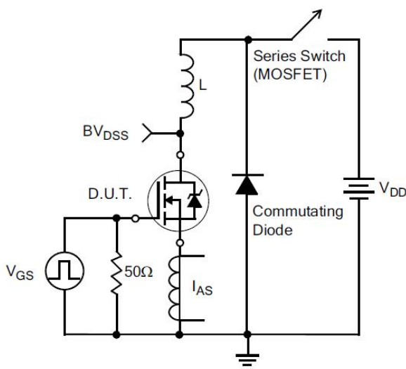
Figure 20. Unclamped Inductive Switching Test Circuit
