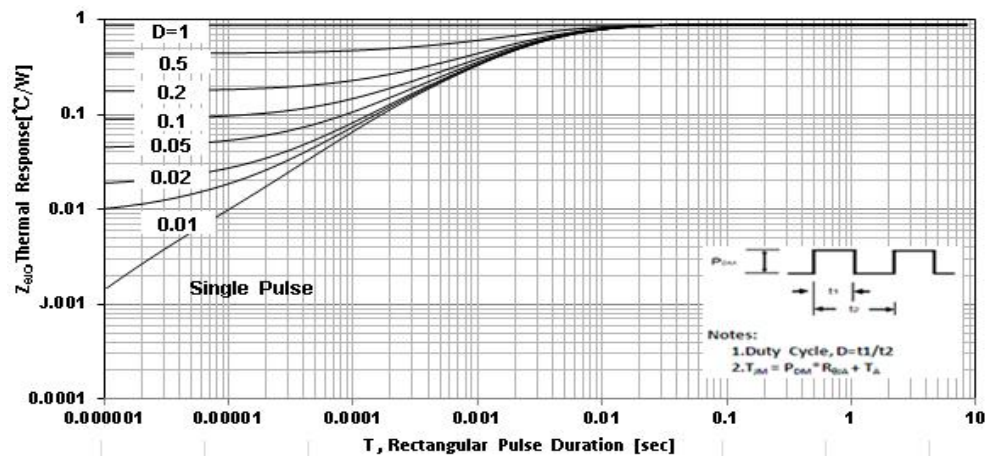
Figure.5 Effective Thermal Impedance, Junction to Case
