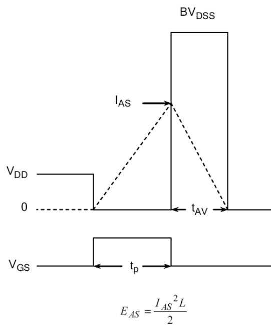
Figure 24. Unclamped Inductive Switching Waveforms
