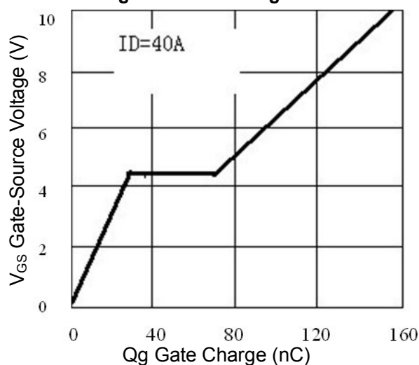
Figure7. Gate Charge
