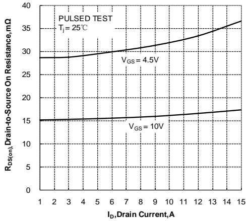
Figure 8. Drain-to-Source On Resistance vs Drain Current
