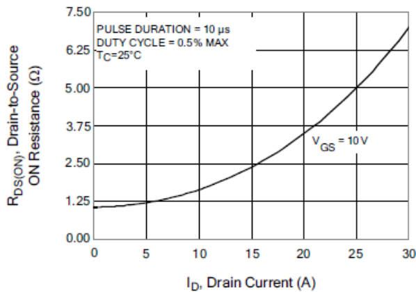
Figure 9. Typical Drain-to-Source Resistance vs Drain Current
