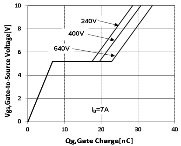
Figure 13 Typical Gate Charge vs Gate to Source Völtage
