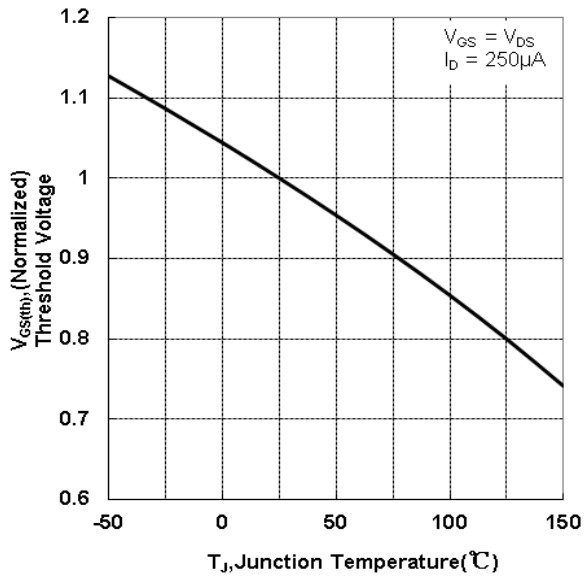
Figure 10 Typical Theshold Völtage vs Junction Temperature
