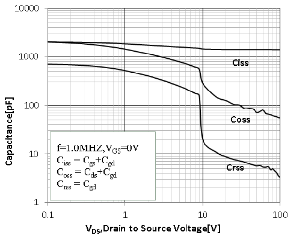
Figure 12 Typical Capacitance vs Drain to Source Völtage
